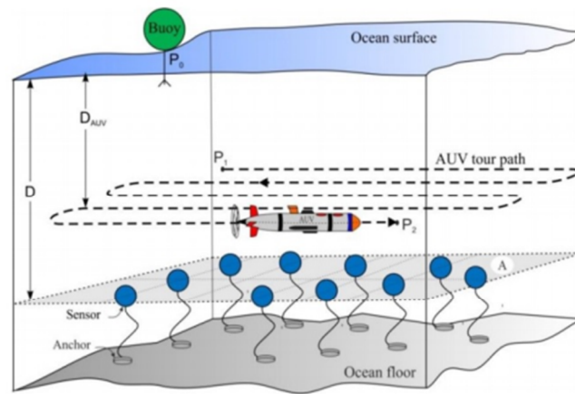
Figure 1-17. AUV Based UWSN Network [33]. AUV is used to collect the data from the sensor nodes which are anchored to the bottom of the sea. When AUV finishes collecting data it transfers the data to the surface station.
