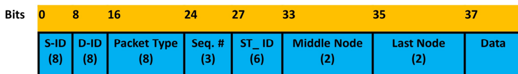
Figure 3-15. Packet Header Format.
